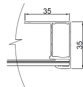
Frame Cross Section
